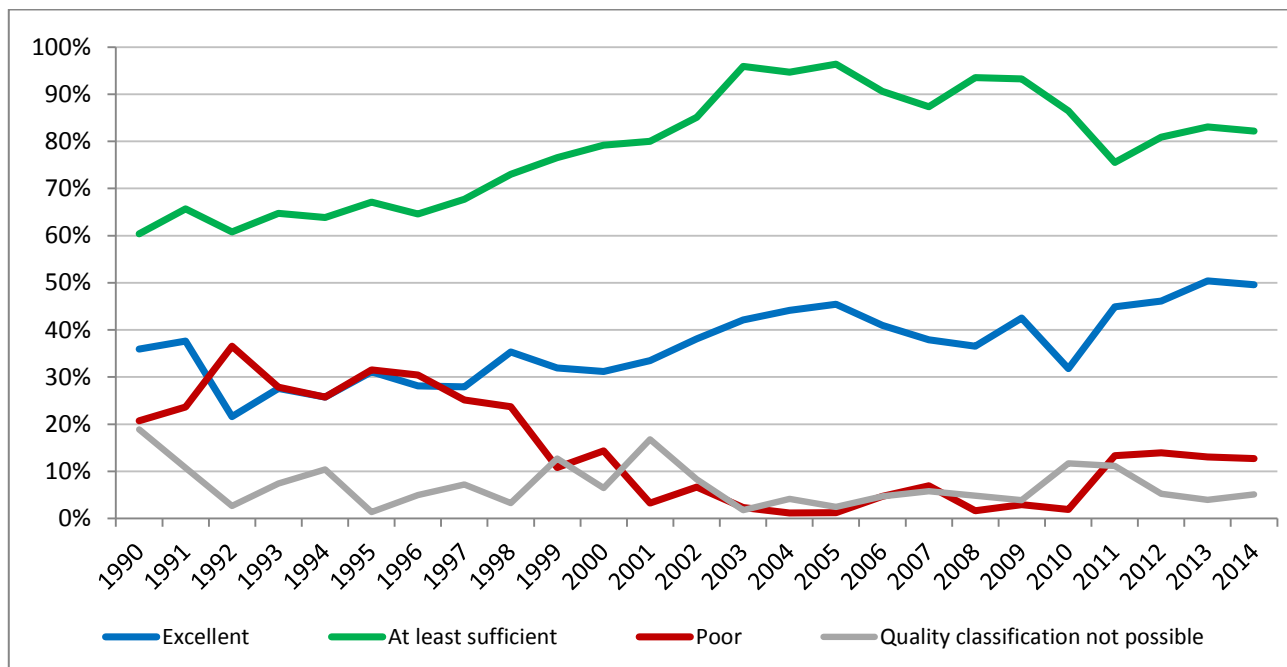
Figure 2: Inland bathing water quality trend in Spain. Note: the “At least sufficient” class also includes bathing waters of “Excellent” quality class, the sum of shares is therefore not 100%.
