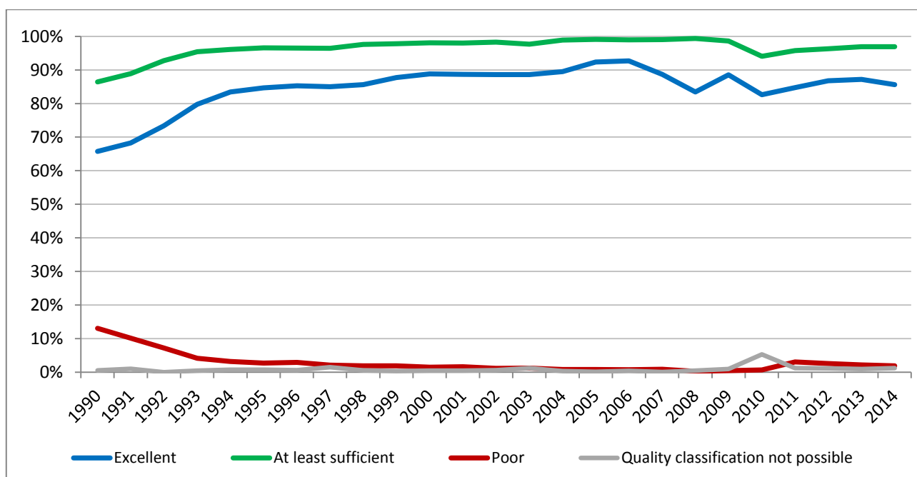
Figure 1: Coastal bathing water quality trend in Spain. Note: the “At least sufficient” class also includes bathing waters of “Excellent” quality class, the sum of shares is therefore not 100%.
