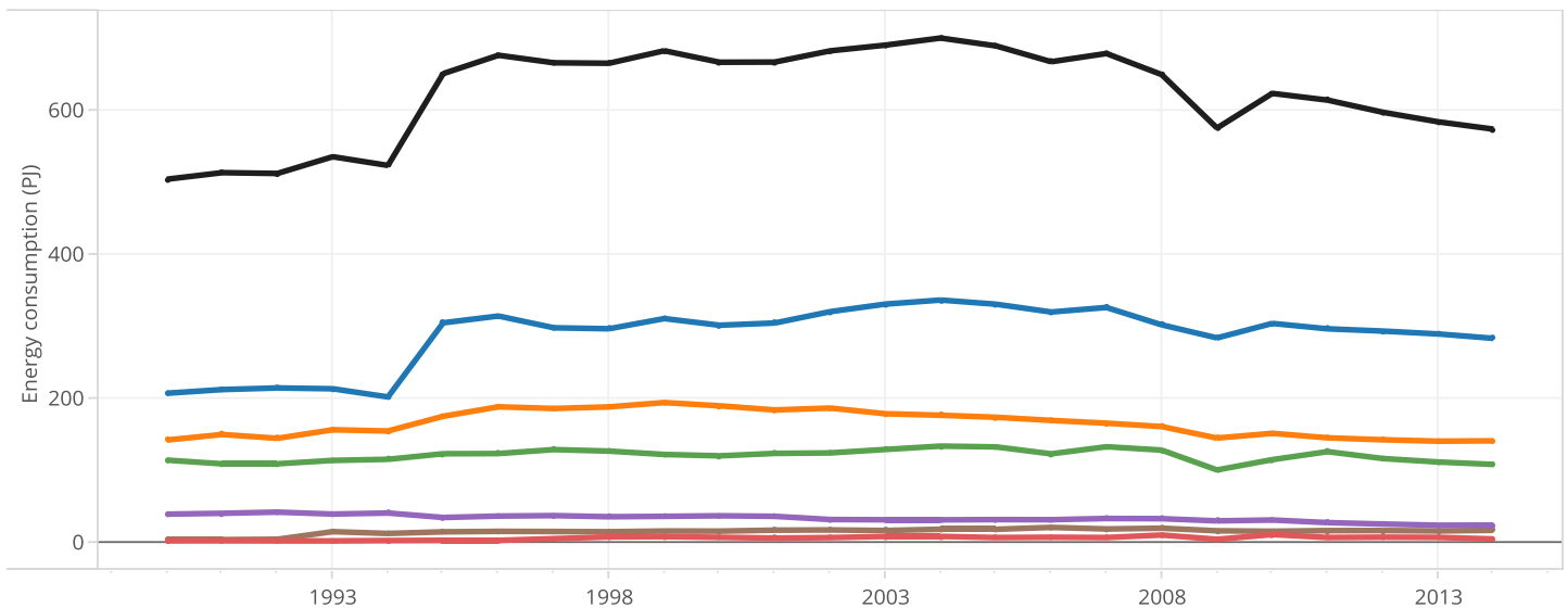
Figure 4. Evolution of the energy consumption of industry in the Netherlands, in petajoules (PJ), for 1990-2014
