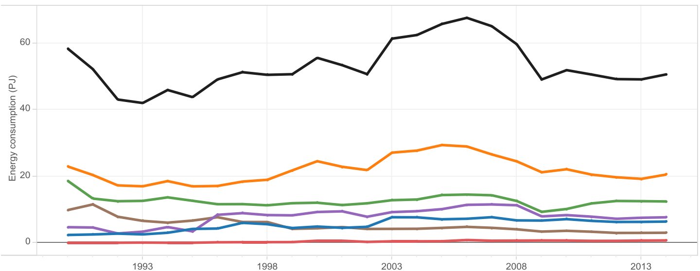
Figure 4. Evolution of the energy consumption of industry in Slovenia, in petajoules (PJ), for 1990-2014
