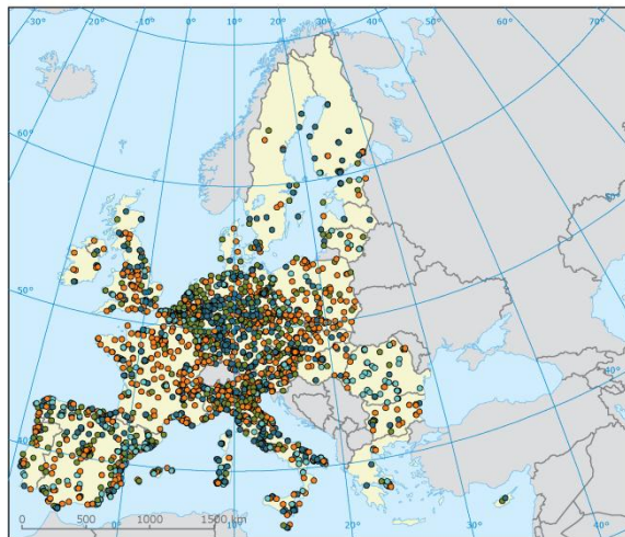
Location, type and number of stations for which 2011 air quality data for nitrogen dioxide (NO 2 ) have been reported (EU-27)
