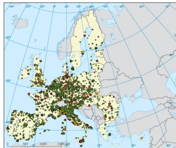
Annual mean nitrogen dioxide (NO 2 ) 2011 and number of stations, based on daily averages with percentage of valid measurements >= 75% in µg/m 3 (EU-27)
