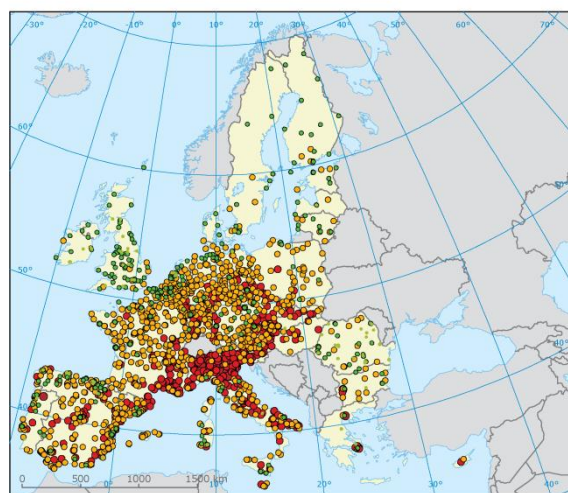
Percentile 93.2 (P93.2) of the daily maximum 8-h average O 3 series with percentage of valid measurements >= 75% in µg/m 3 over the year and number of stations (EU-27)
