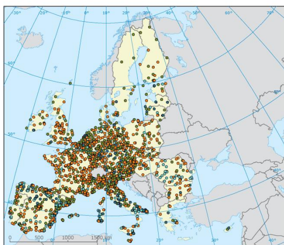
Location, type and number of stations for which 2011 air quality data for ozone (O 3 ) have been reported (EU-27)
