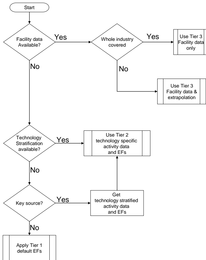
Figure 3.1 Decision tree for source category 2.D.3.c Asphalt roofing
