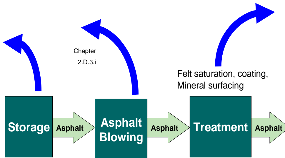
Figure 2.1 Process scheme for source category 2.D.3.c Asphalt roofing
