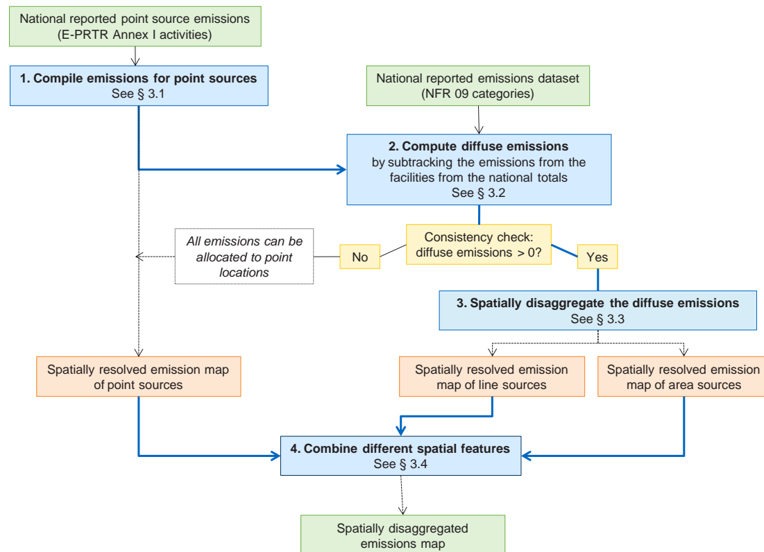
Figure 3-1 General approach for compiling a spatial emission inventory
