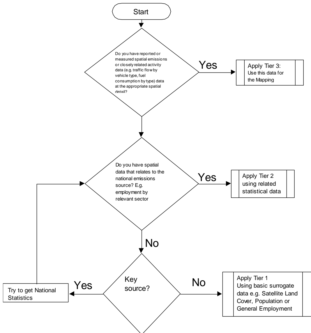
Figure 3-2 General decision tree for emissions mapping
