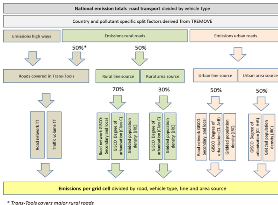
Figure 3-3 Overview of the applied methodology for the spatial distribution of the road transport, Theloke et al. (2009).
