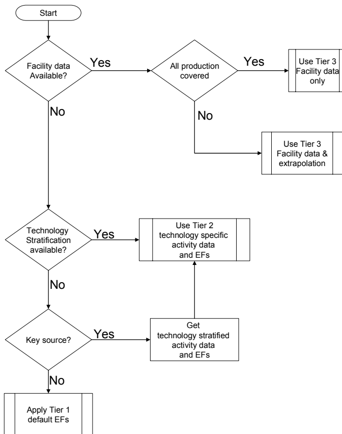
Figure 3.1 Decision tree for source category 2.C.5.a Copper production
