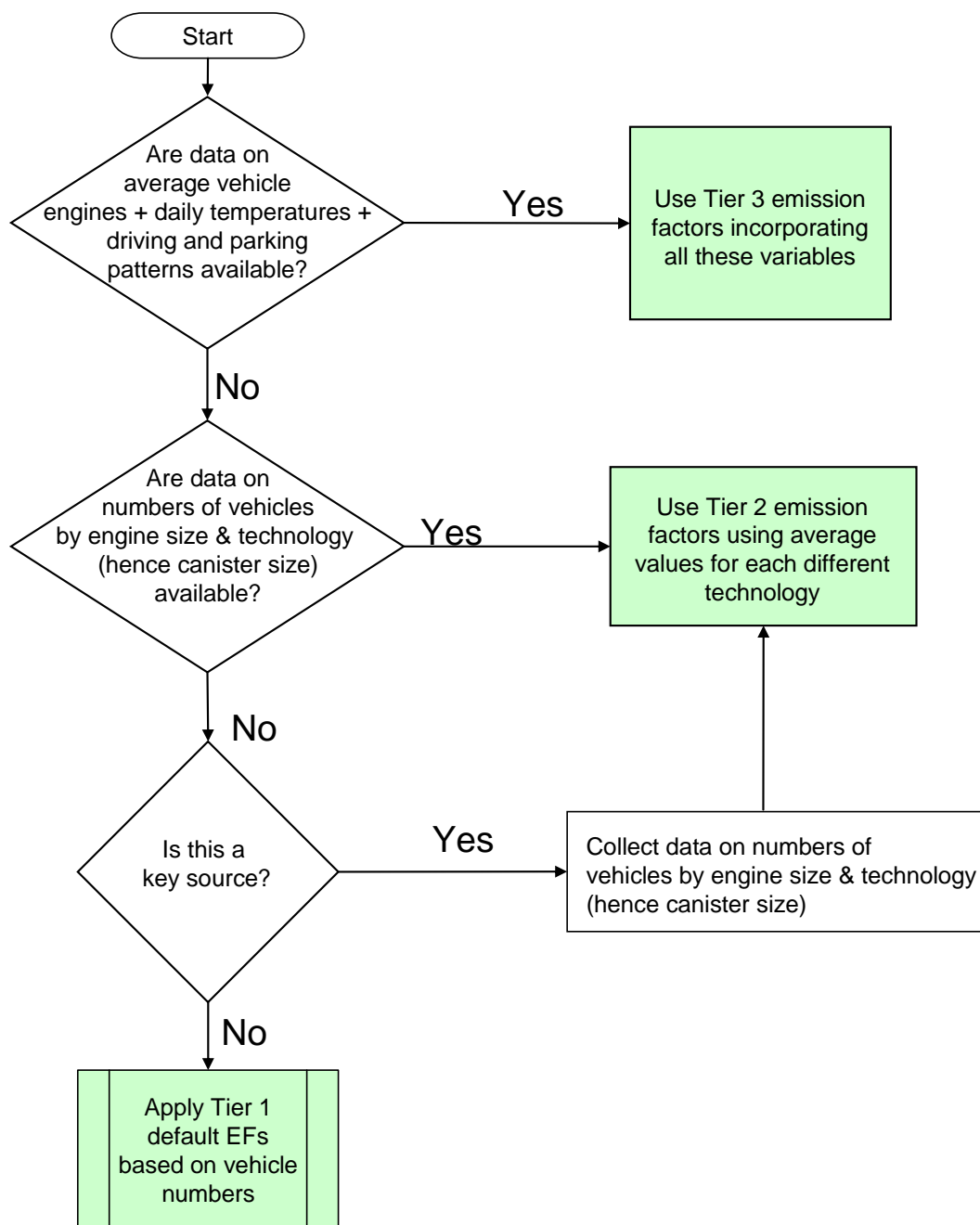
Figure 3-1 Decision tree for evaporative emissions
