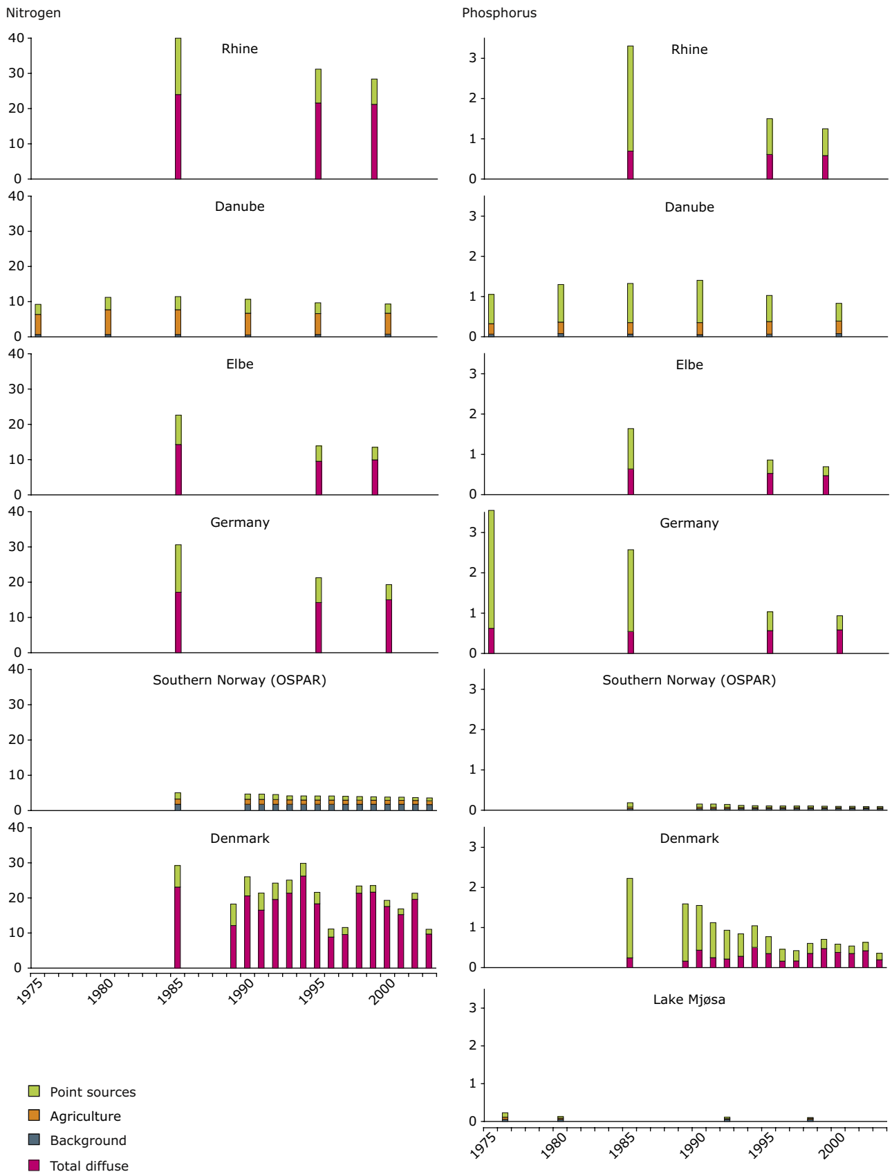
Figure 7.1 Long time series of source apportioned load of nitrogen and phosphorus (kg/ha/year on y axes) in the period 1975–2003 (mixed approaches)
