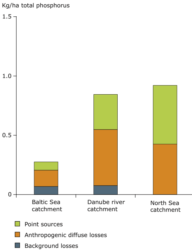
Figure 2 Source apportionment of annual phosphorus load
