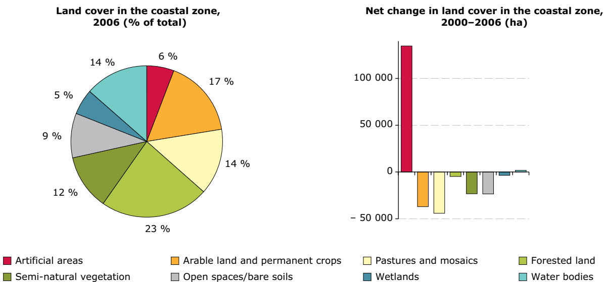
Figure 2.3 Land cover 2006 (left), and net change in land cover 2000–2006 (right) in coastal zones of 28 coastal countries *
