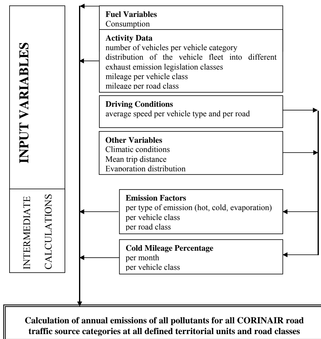
Figure 5.1: Flow chart of the application of the baseline methodology
