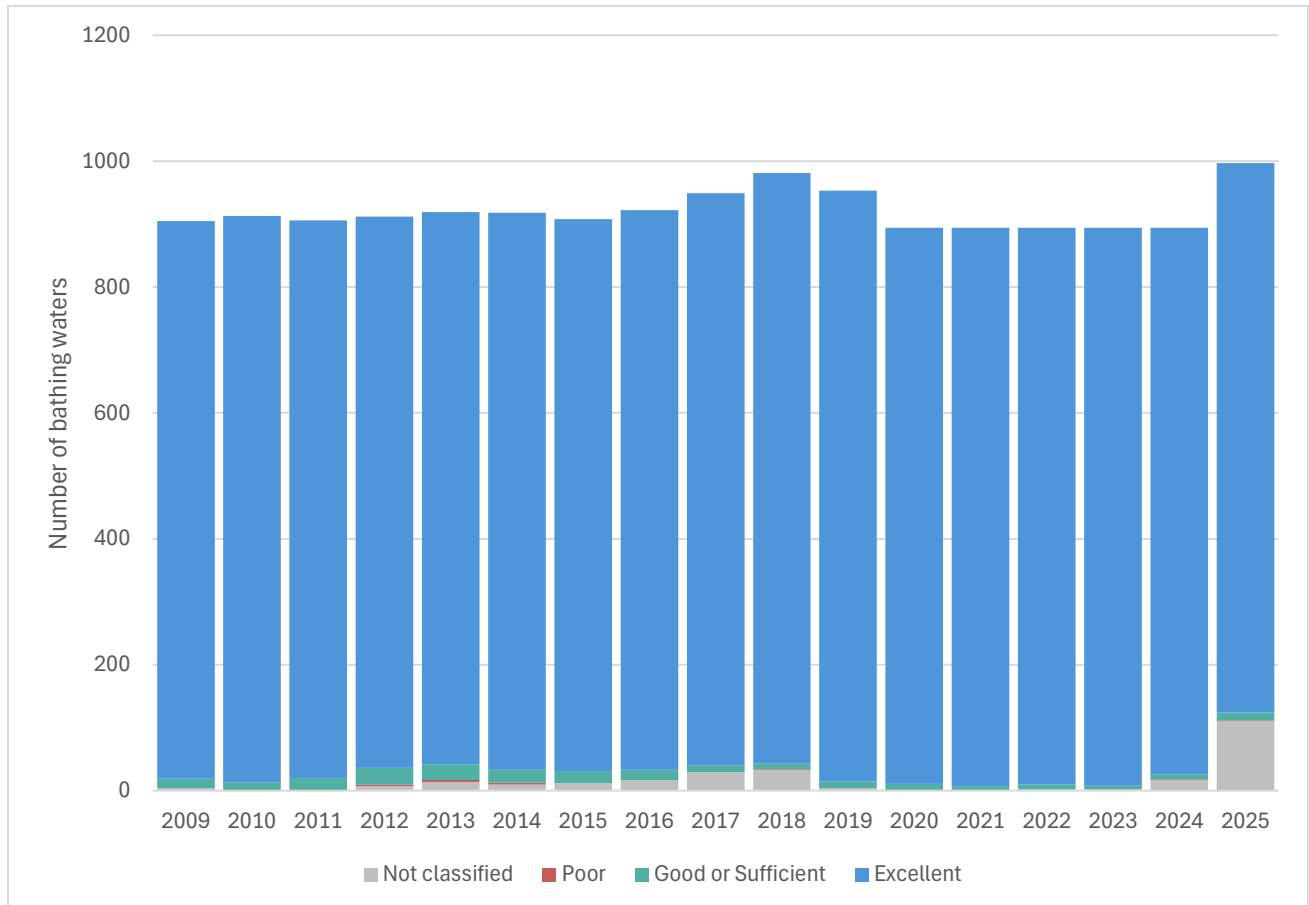
Figure 1: Trend of coastal bathing water quality. Notes: Each column represents an absolute number of bathing waters in the season. Quality classes “good” and “sufficient” are merged for comparability with the classification of the preceding Bathing Water Directive 76/160/EEC.
