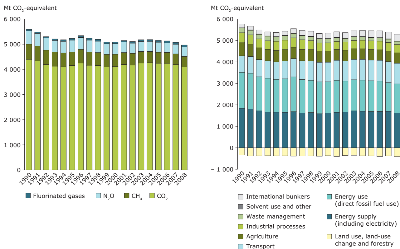
Figure 3.4 Total EU GHG emissions by sector and by gas, 1990–2008
