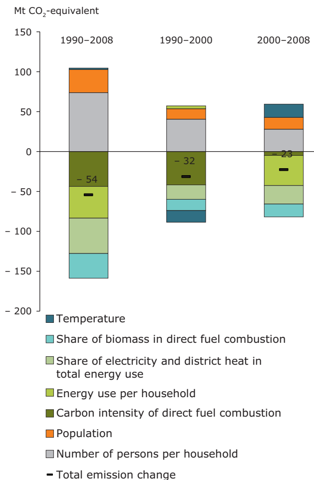
Figure 7.15 Decomposition analysis of direct CO 2 emission trends from EU households, 1990–2008
