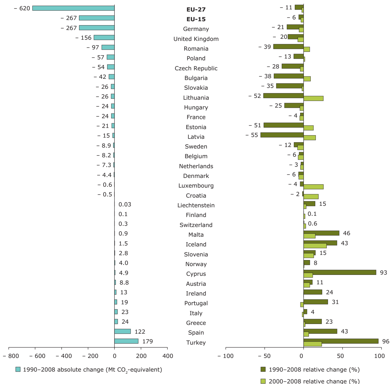
Figure 3.5 Absolute change and average annual relative change of total GHG emissions in the EU, 1990–2008
