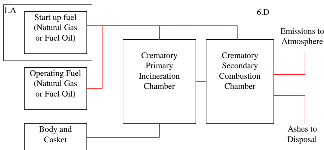
Figure 2-1 Flow diagram of the cremation process showing activities included in this chapter
