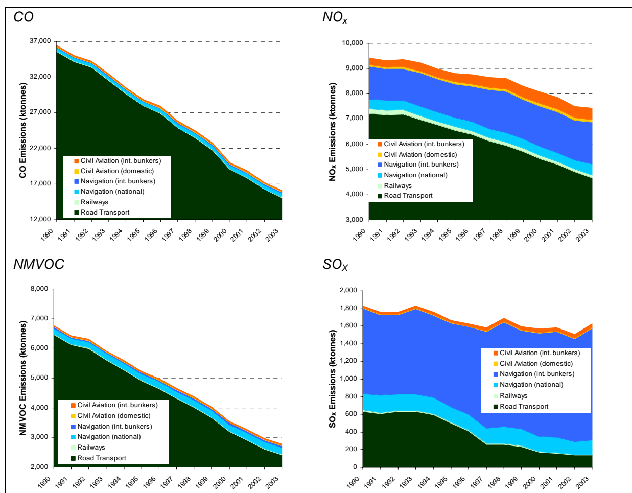
Figure 7: Emission trends of air pollutants (CO, NMVOC, NO x and SO x ) by transport type in the EEA32, 1990 –2003
