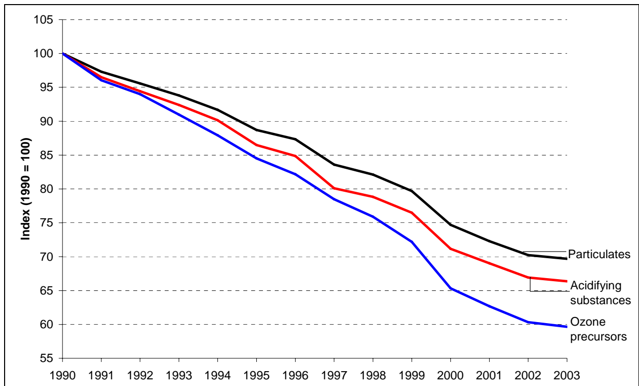
Figure 1: Transport emissions of air pollutants for EEA32 (acidifying substances, ozone precursors and particulates), 1990-2003 (indexed: 1990 = 100)
