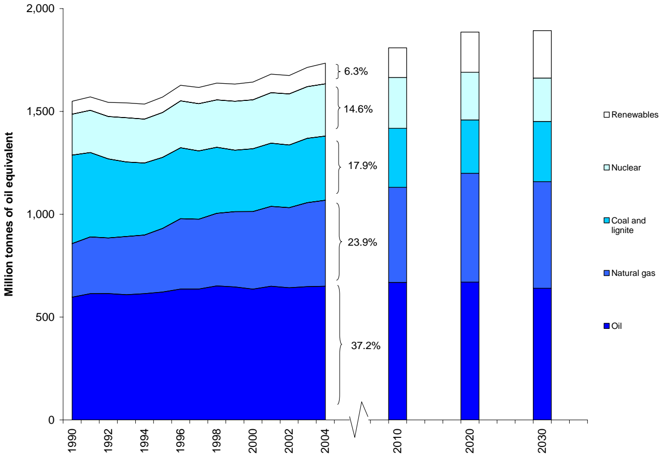
Fig. 1a: Total energy consumption by fuel, EU-25
