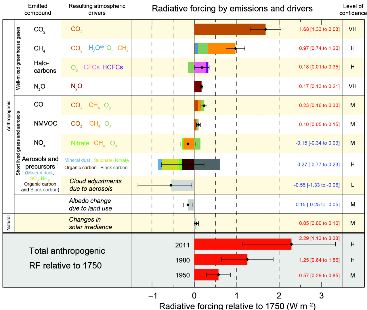
Figure 2: Radiative forcing estimates in 2011 relative to 1750 and aggregated uncertainties for the main drivers of climate change
