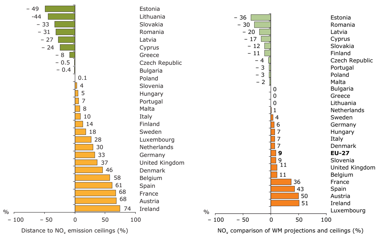
Figure 4 Proximity to NO x emission ceilings for year 2006 (left) and comparison of WM projections reported by Member States with their respective ceilings (right)
