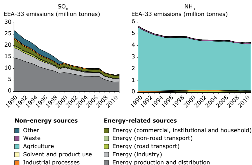
Figure 6.5 EEA-33 emissions of selected air pollutants by main source sectors, 1990–2011 (cont.)
