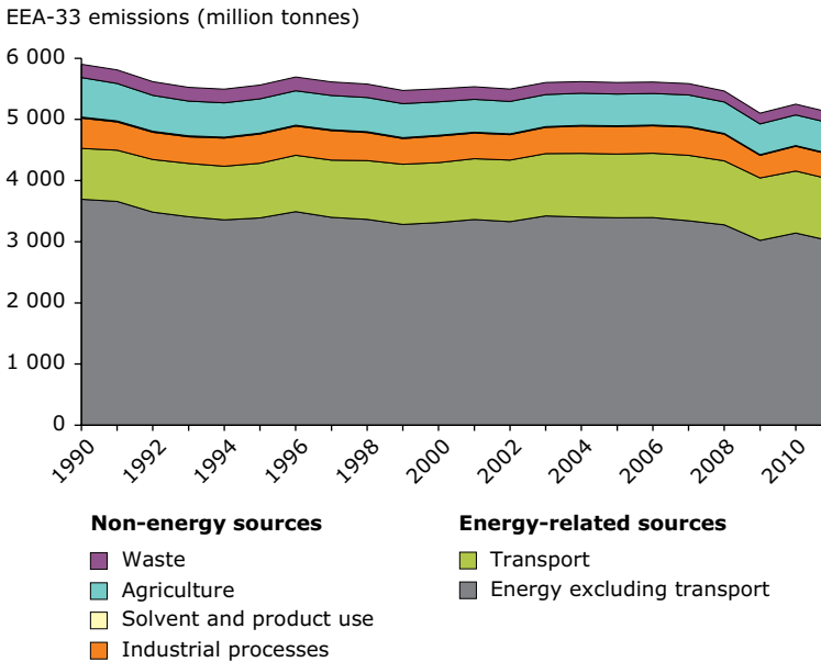
Figure 6.6 EEA-33 emissions of greenhouse gases by main source sectors, 1990–2011
