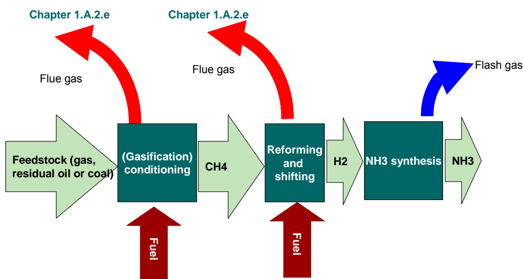
Figure 2.3 Simplified process scheme of ammonia production
