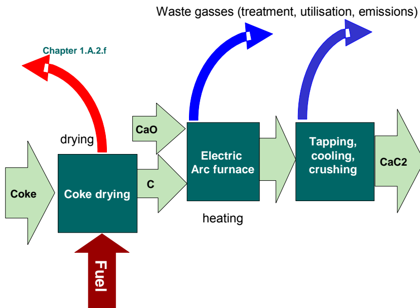
Figure 2.5 Simplified process scheme of calcium carbide production (EC, 2006c; EPA, 1993)
