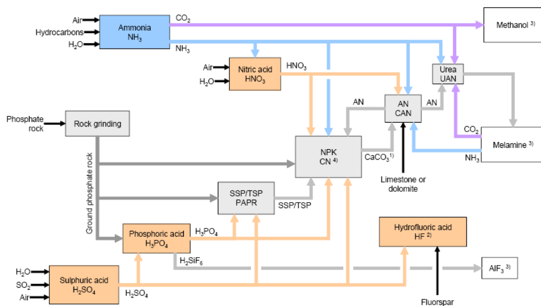
Figure 2.2 Overview of boundaries and links between the LVIC-AAF industries
