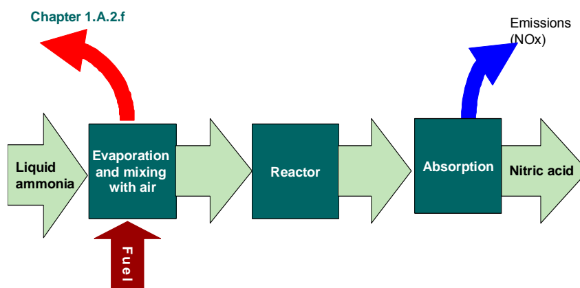
Figure 2.4 Simplified process scheme of nitric acid production
